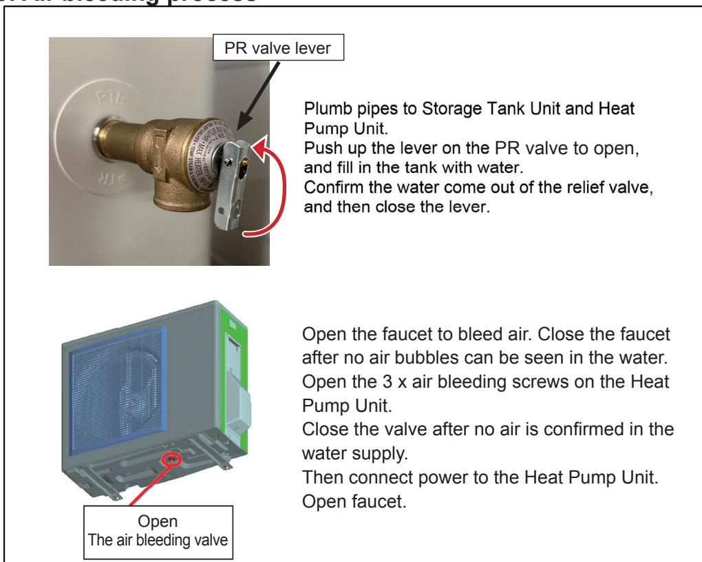
Figure 3: Air bleeding process
