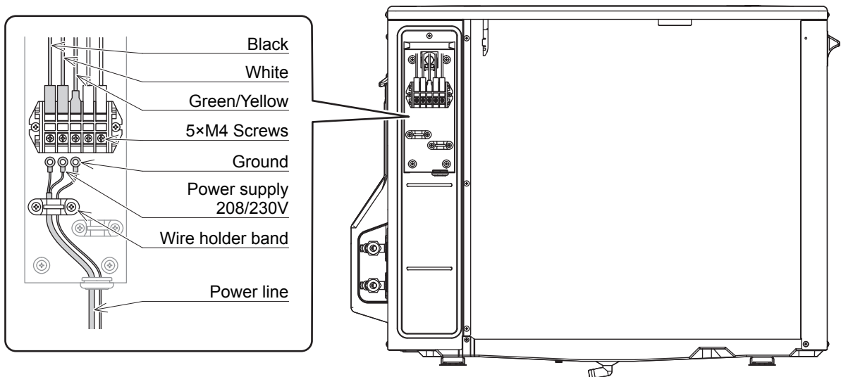
Figure 4: Connect power
